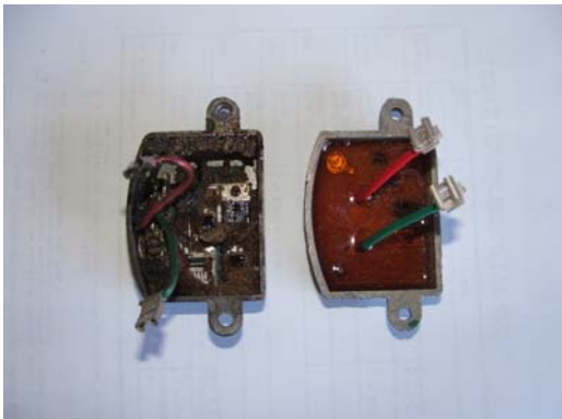
Melted regulator left, new regulator right
